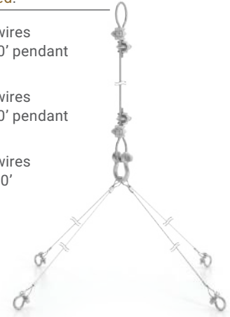
Shackles | quick links | aircraft cable.
