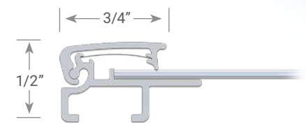
SupraSlim Profile
